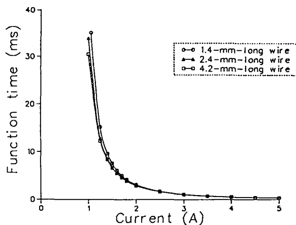
Fig. 4. Calculated function times for three bridgewire lengths. The wire diameters were 0.051 \text{ mm} , and the HMX density was 1.64 \text{ g/cm}^3 .
