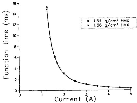
Fig. 13. Calculated function times for two HMX loading densities are shown. A 1.4-mm-long and 0.051-mm-diam bridgewire was used.
