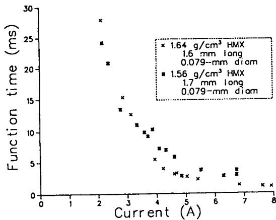
Fig. 16. Experimentally measured function times for two HMX loading densities are shown.
