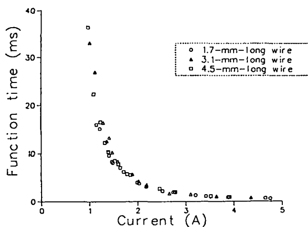
Fig. 3. Experimentally measured function times for three bridgewire lengths. The wire diameters were 0.051 \text{ mm} , and the HMX density was 1.64 \text{ g/cm}^3 .
