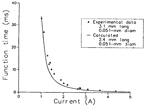
Fig. 6. Comparison of experimental and calculated function times. The HMX density was 1.64 \text{ g/cm}^3 .
