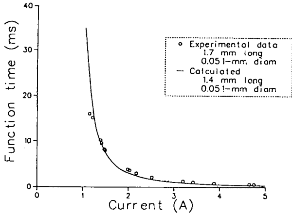
Fig. 5. Comparison of experimental and calculated function times. The HMX density was 1.64 \text{ g/cm}^3 .
