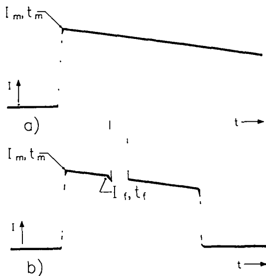
Fig. 1. Reproduction of oscilloscope current-time histories for an ER-322 device (a) that fails to function and (b) that functions.
