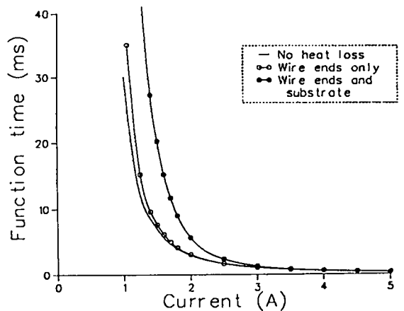
Fig. 17. Calculated time-to-ignition for three modes of heat loss from the bridgewire. The modeled bridge is 1.4 mm long and 0.051-mm diam, and the HMX loading is 1.64 \text{ g/cm}^3 .
