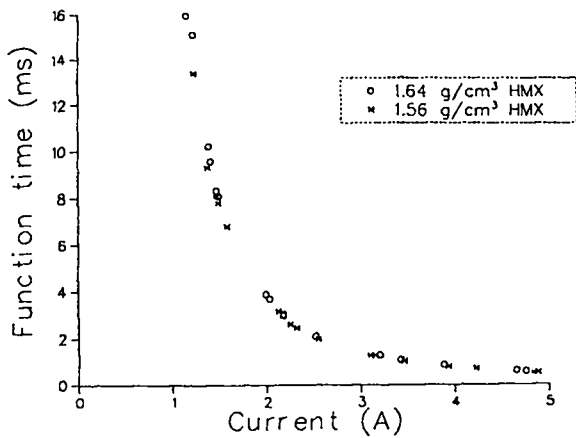
Fig. 12. Experimentally measured function times for two HMX loading densities are shown. The bridgewires were 1.7 mm long and 0.051-mm diam.
